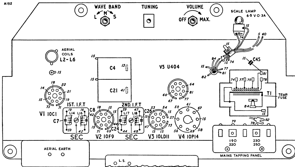
The layout of the top of the chassis
